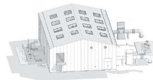
Drawing of Influent Pump Station
